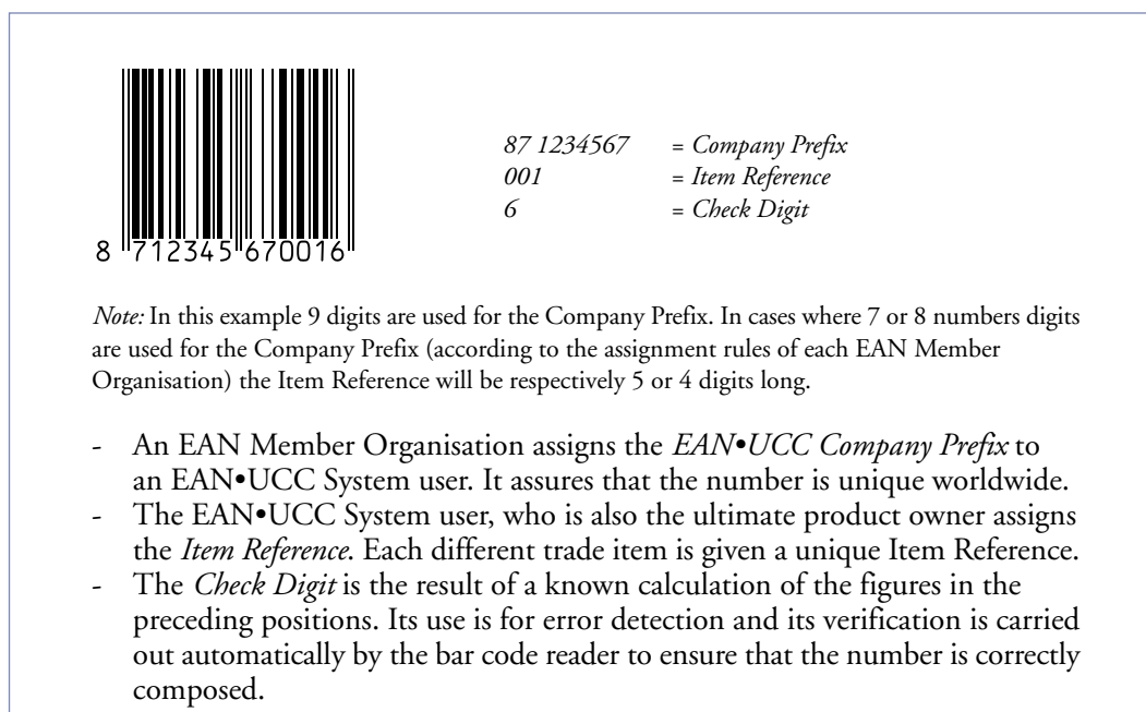
Figure 2: Numeric Construction of the EAN-13 bar code
